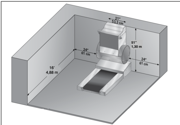
Misure minime vasca
